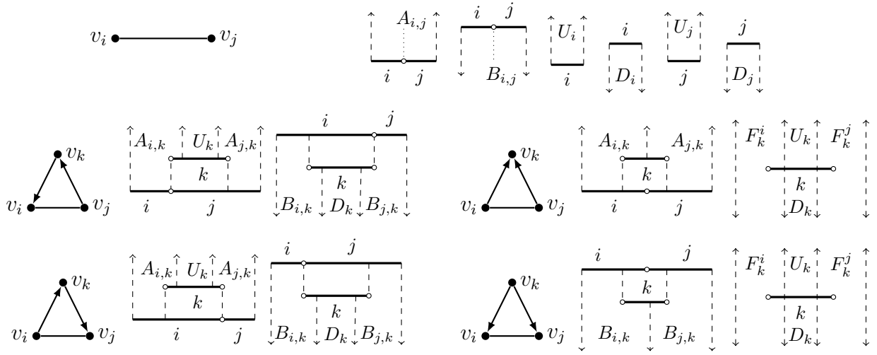
Figure 3.4: The case C_{i,j} = \{A_{i,j}, B_{i,j}\} .
