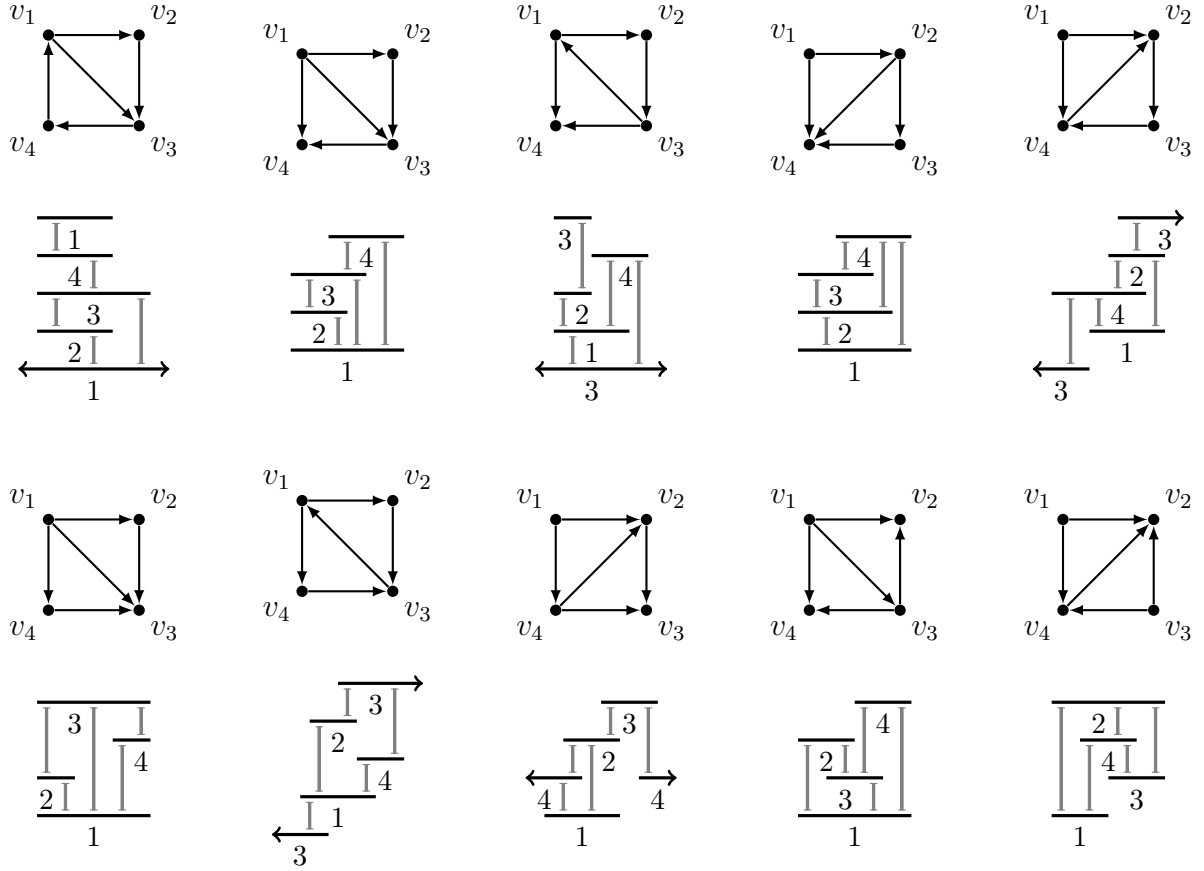
Figure 4.4: Layouts of digraphs with four vertices and five edges.
