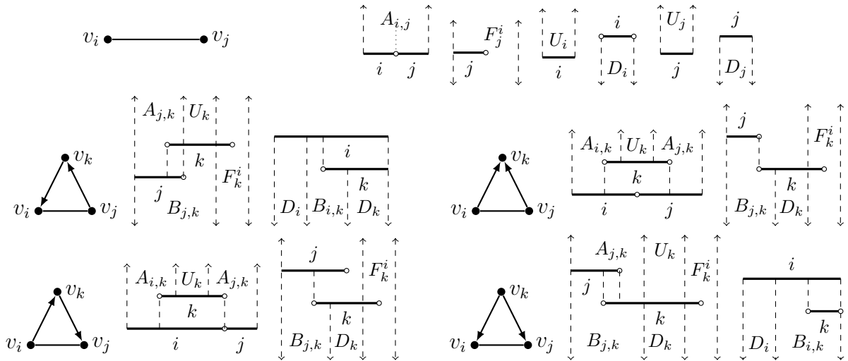
Figure 3.5: The case C_{i,j} = \{A_{i,j}, F_j^i\} .
