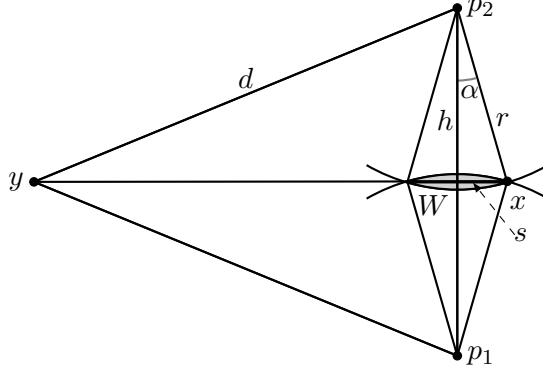
Figure 5.2: Determining the area of W = W(x, y; r) .
