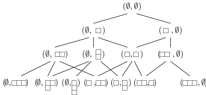
Figure 2. Bratteli Diagram of A_k(u_1, u_2; q) and R_k(q)
