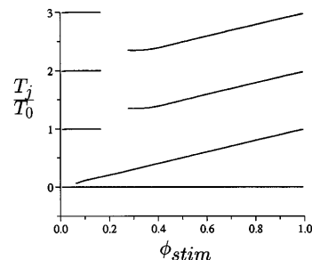
FIG. 2. Summary of resetting data for reentrant excitation using a suprathreshold stimulus. The normalized excitation times T_j/T_0 at position 0.75 are displayed as a function of the phase of stimulation of the reentrant wave. Stimuli either have little effect 0 \leq \phi < 0.16 , lead to annihilation, 0.16 < \phi < 0.28 , or reset the oscillation, 0.28 < \phi < 1 .
