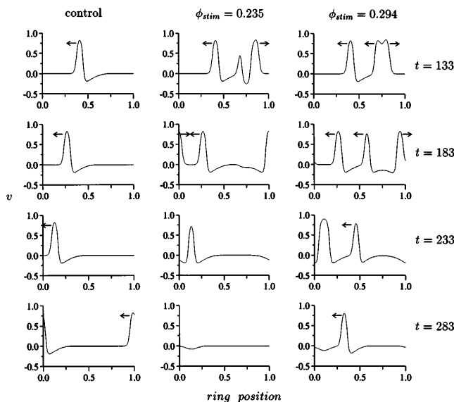
FIG. 1. Simulation of the Fitzhugh-Nagumo equation showing propagation of excitation around a ring. The ring circumference is about 4.47 cm. We display the normalized position from an arbitrary origin. In each panel the v variable is displayed as a function of ring position. Each row corresponds to the activity shown at the time shown to the right of the row, where t = 0 corresponds to the time the excitation is at position 0.75 before stimulation. Column 1: no stimulus; column 2: stimulus delivered at position 0.75 at \phi_{stim} = 0.235 . A single wave is generated that propagates in a retrograde direction. The collision of this wave with the original reentrant wave leads to annihilation of the reentrant wave. Column 3: stimulus delivered at position 0.75 at \phi_{stim} = 0.294 . Two waves are generated. The retrogradely propagated wave collides with the original wave and leads to its annihilation. The anterogradely propagated wave continues, leading to resetting of activation times at position 0.75.
