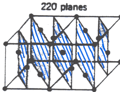
(b) Two unit cells of face-centered cubic lattice (Cubic F)
