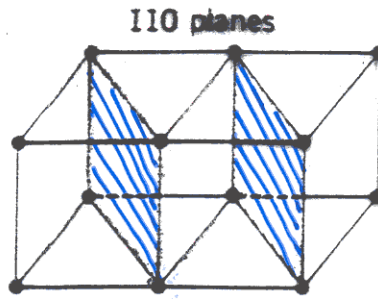
(a) Two unit cells of primitive cubic lattice (Cubic P)
