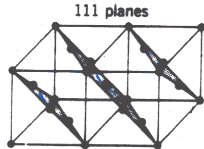
(b) Two unit cells of face-centered cubic lattice (Cubic F)
