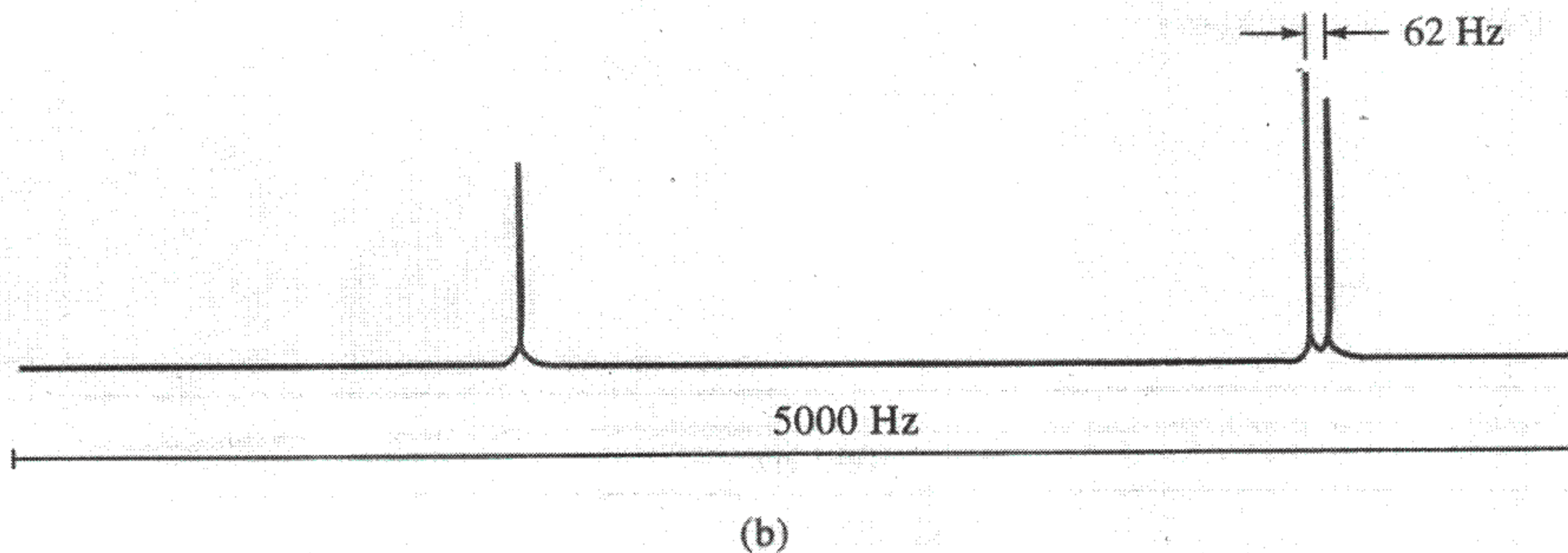
Figure 19-10 (a) FID signal for ^{13}\text{C} in cyclohexane; (b) Fourier transform of (a). (From R. J. Abraham, J. Fisher and P. Loftus, Introduction to NMR Spectroscopy , p. 91. New York: Wiley, 1988. Reprinted by permission of John Wiley & Sons, Inc.)
