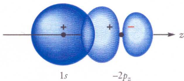
(c) Bonding, \sigma (significant overlap)
