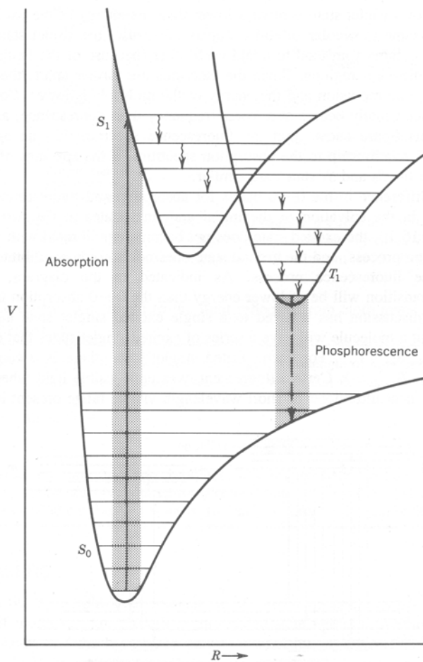
Fig. 16.8 Absorption and phosphorescence by a diatomic molecule. The shaded areas indicate transitions to a range of vibrational quantum numbers.
