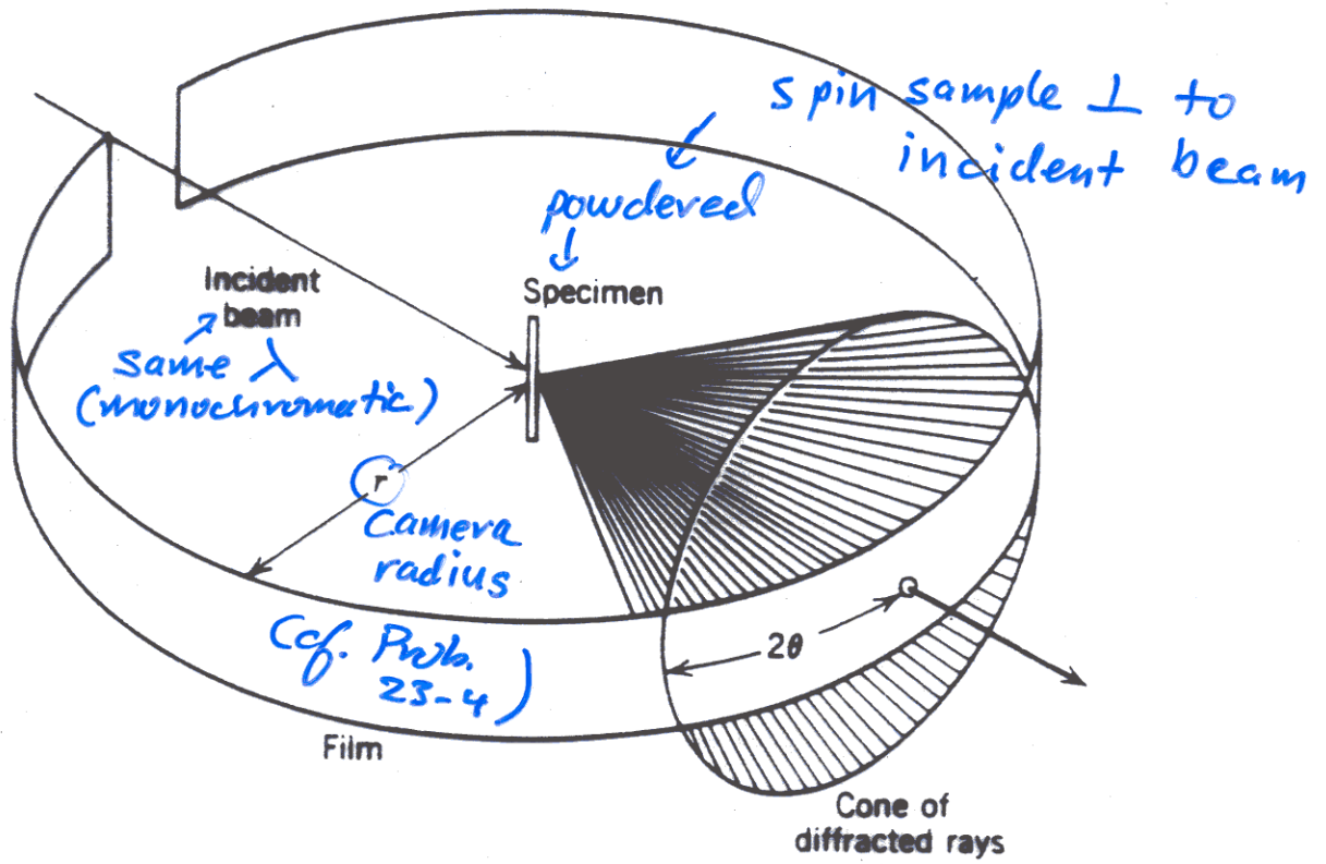
Figure 23.8 X-ray powder camera.
