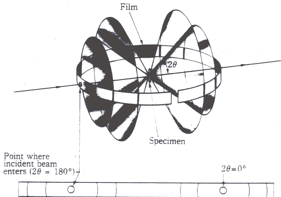
Figure 27.28 Debye-Scherrer powder method.
