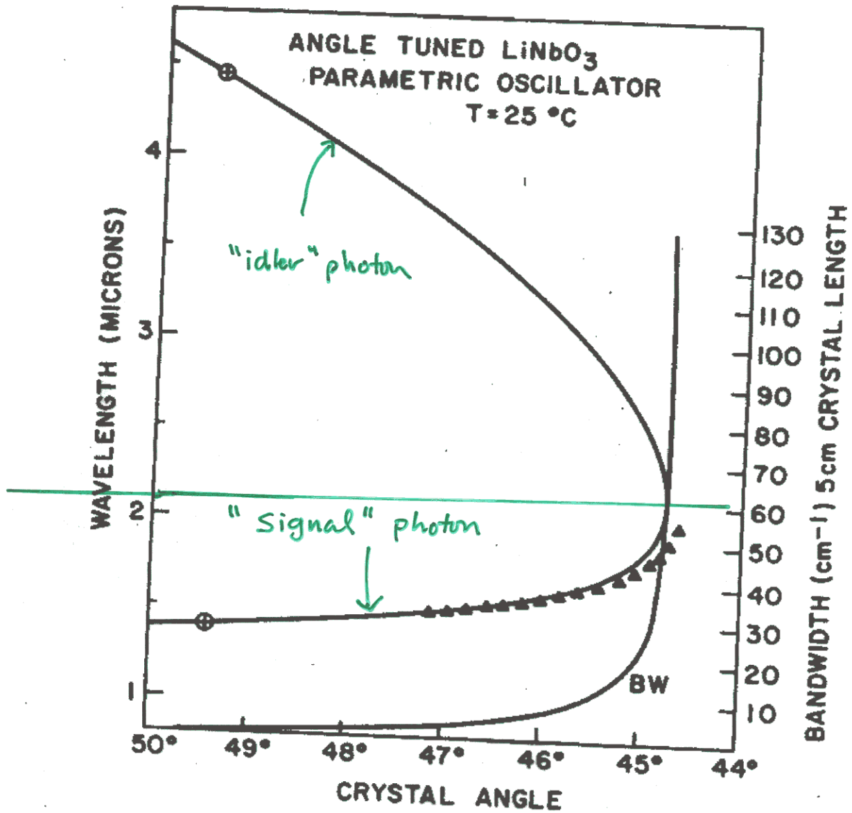
Fig. 2. Angle tuned \text{LiNbO}_3 OPO tuning curve and crystal gain bandwidth.
