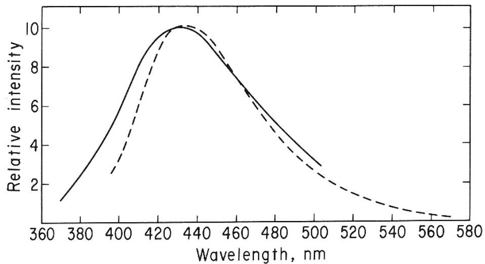
- - - Chemiluminescence Spectrum of Dianion
