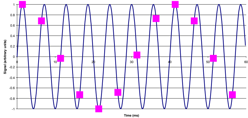
175-Hz Signal Sampled at Only 200 Hz
