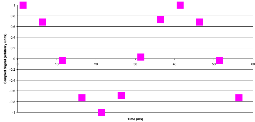
Blowing off Nyquist: Creation of a 25-Hz Alias
