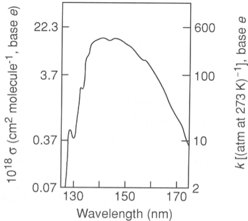
FIGURE 4.2 Absorption coefficients for O 2 in the Schumann–Runge continuum. Note log scale. (Adapted from Inn, 1955.)
