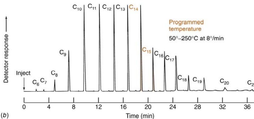
Harris Figure 24-7(b): Same Gas Chromatography Experiment with Column at Increasing Temperature
