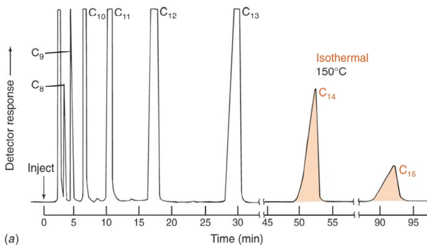
Harris Figure 24-7(a): Gas Chromatography Experiment with Column at Constant Temperature
