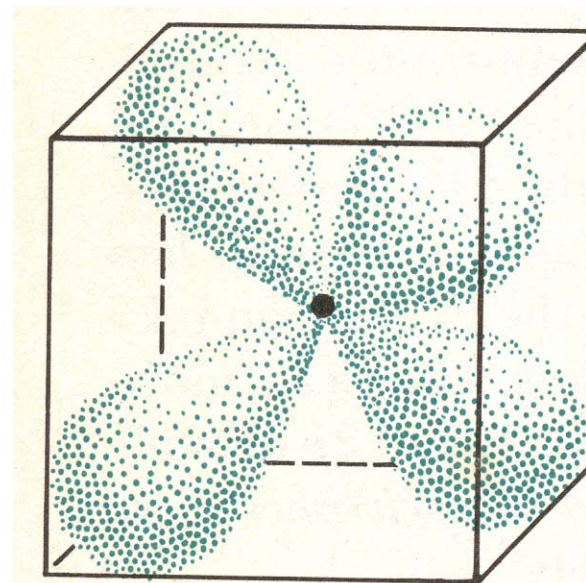
FIG. 5.16 sp^3 hybrid orbitals. (The black dot represents the nucleus.)
