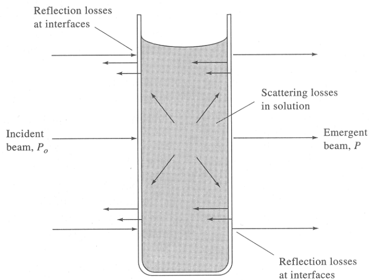
Figure 13-1 Reflection and scattering losses.
