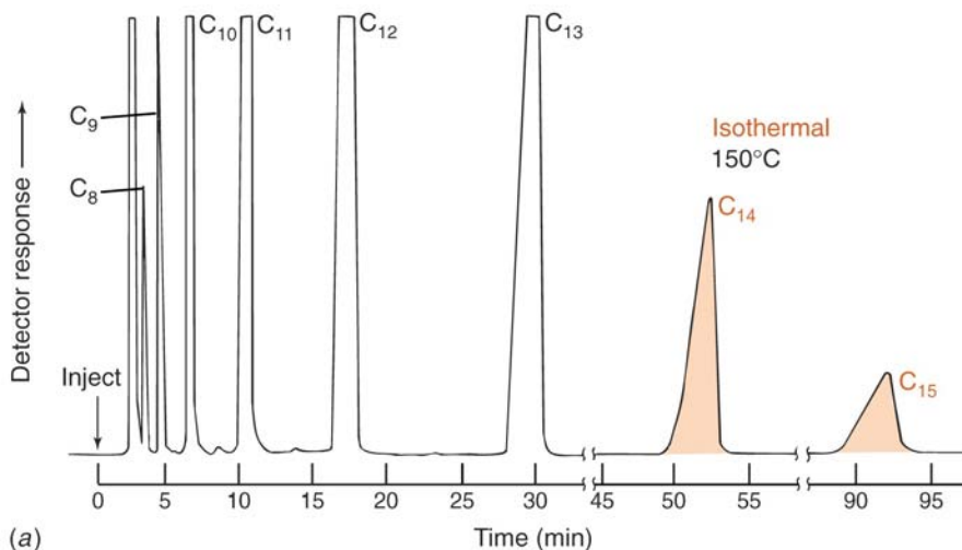
Harris Figure 24-10(a): Gas Chromatography Experiment with Column at Constant Temperature
