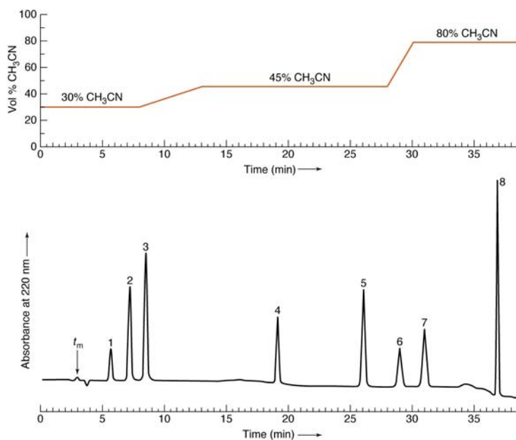
Harris Figure 25-13: Same Liquid Chromatography Experiment with Mobile Phase of Changing Composition (“gradient elution”)
