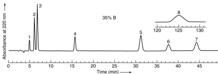
Harris Figure 25-12: Liquid Chromatography Experiment with Mobile Phase of Constant Composition (“isocratic elution”)
