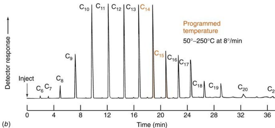
Harris Figure 24-10(b): Same Gas Chromatography Experiment with Column at Increasing Temperature
