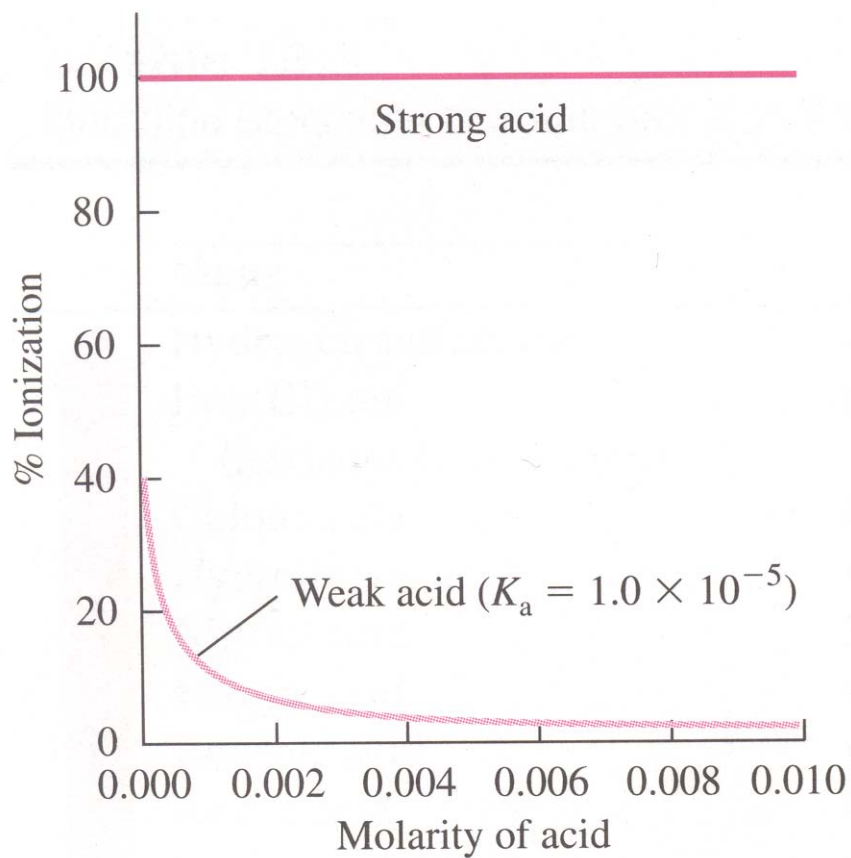
● Figure 15.5 Percent ionization as a function of molarity.
