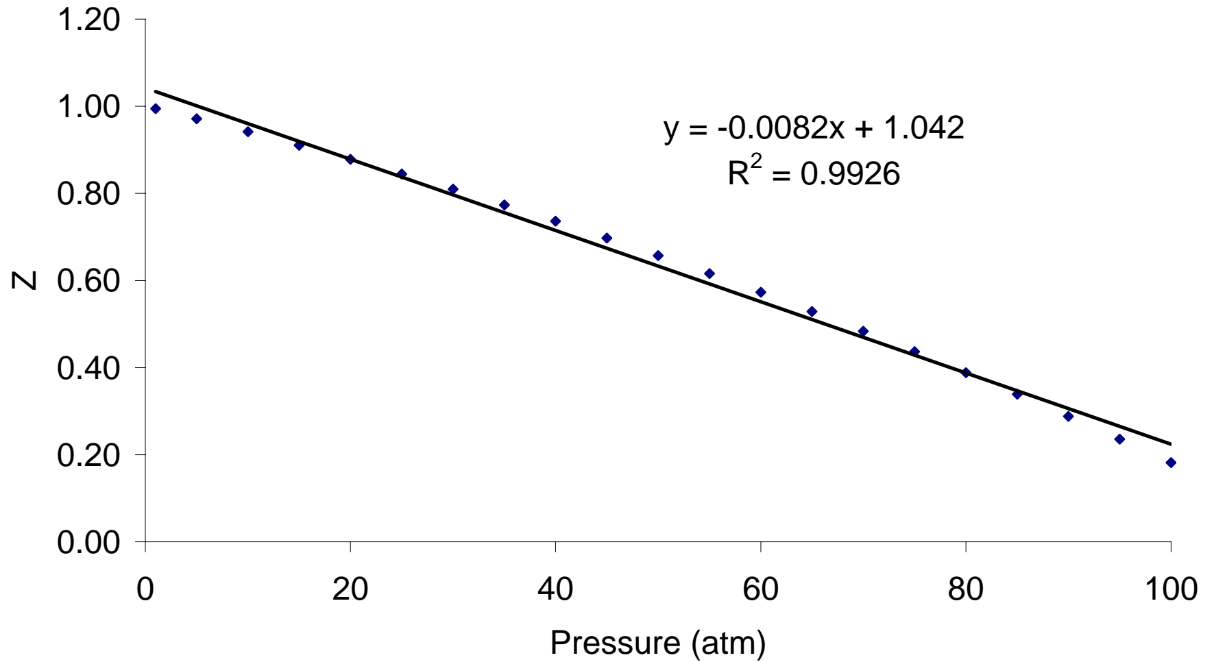
Compression Factor for N 2 at 150 K Linear Fit ( Z = 1 + B'p )
