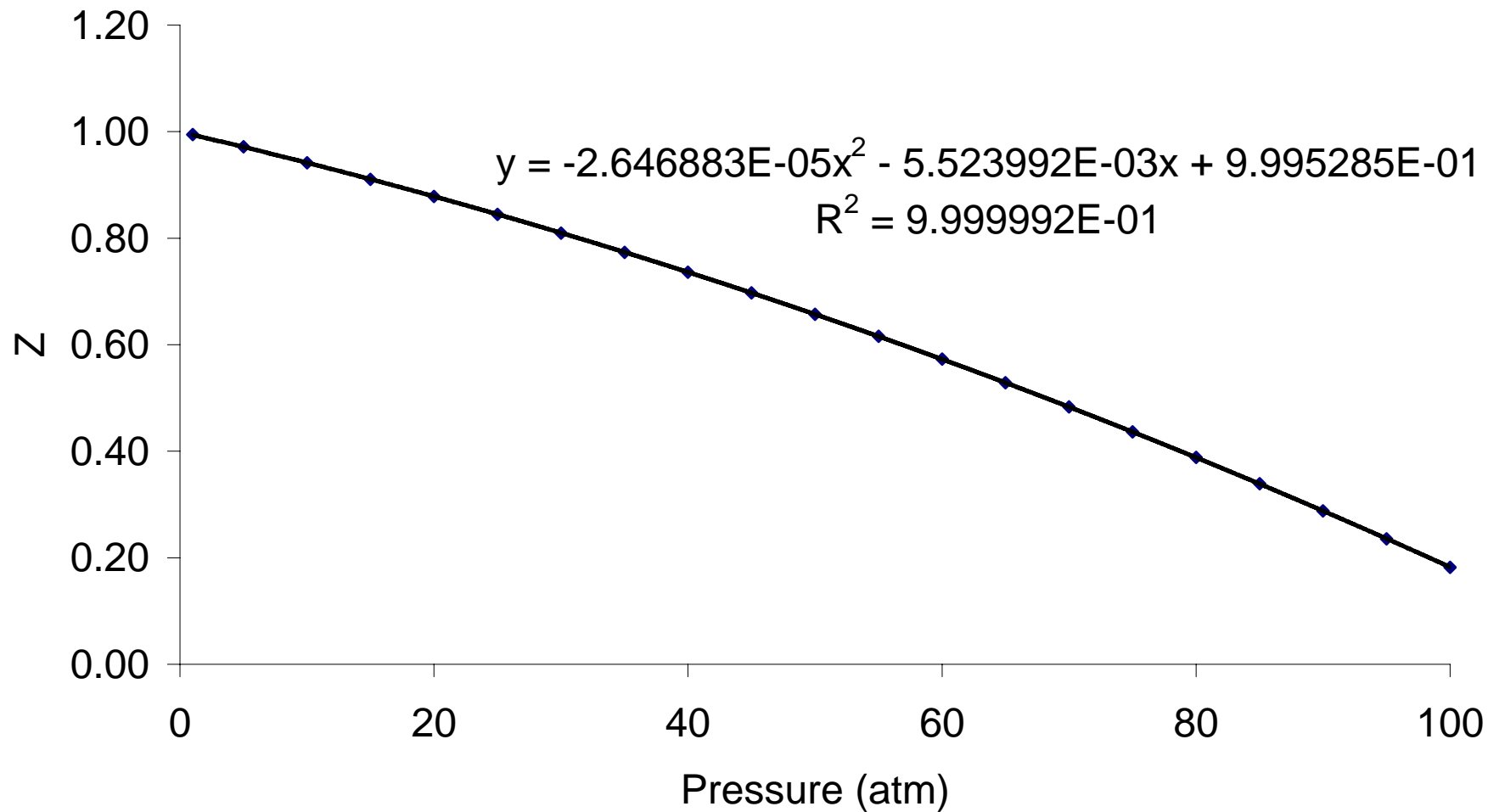
Compression Factor for N 2 at 150 K (Quadratic Fit: Z = 1 + B'p + C'p^2 )
