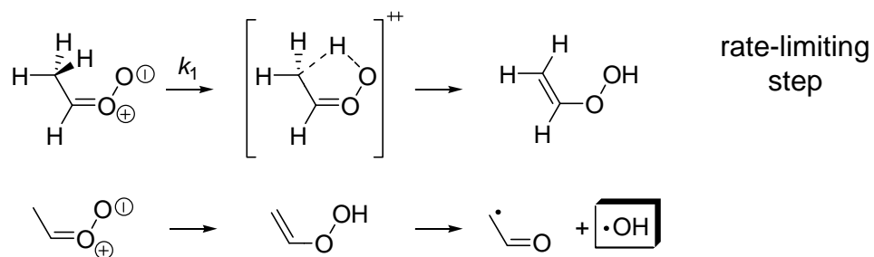
Predicted Values of the 1,4-Hydrogen Shift Rate Constant
