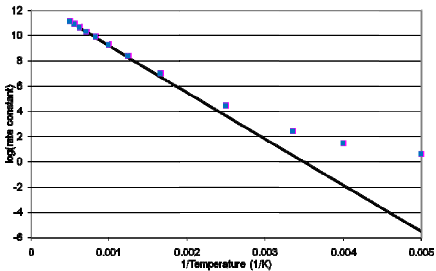
Predicted Values of the 1,4-Hydrogen Shift Rate Constant
