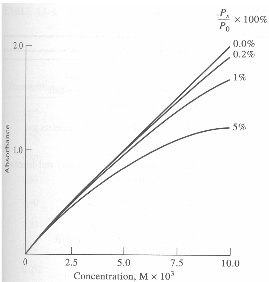
Figure 13-6 Apparent deviation from Beer's law brought about by various amounts of stray radiation.
