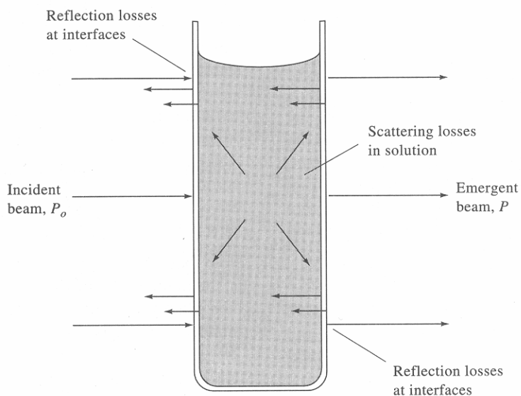
Figure 13-1 Reflection and scattering losses.
