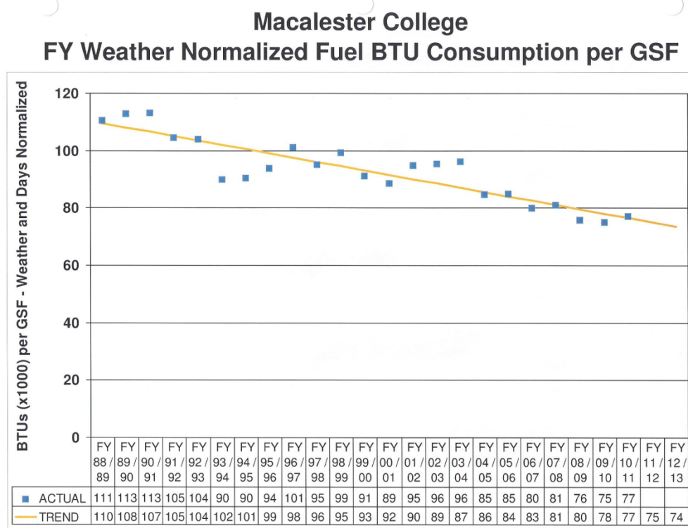
Figure 4: Weather Normalized Fuel BTU Consumption per GSF
